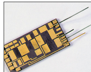
Fine wire to pad
