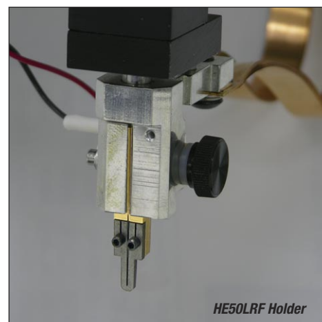
HE50RF Holder
