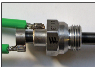
Crimp weld connector
