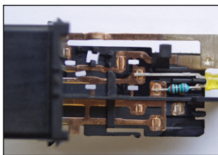
Projection weld switch dashboard
