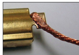
Pre compacted wire to terminal
