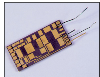
Welding fine wire to pad
